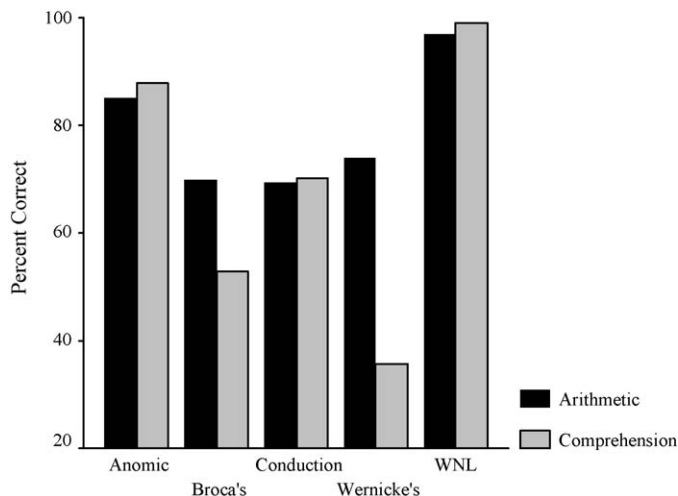
Fig. 2. Arithmetic and comprehension performance across aphasia subgroups. WNL = within normal limits on the Western Aphasia Battery; conduction = conduction aphasia. The sample sizes were as follows: anomic ( n = 14 ), Broca's ( n = 17 ), conduction ( n = 6 ), Wernicke's ( n = 7 ), and WNL ( n = 19 ).
