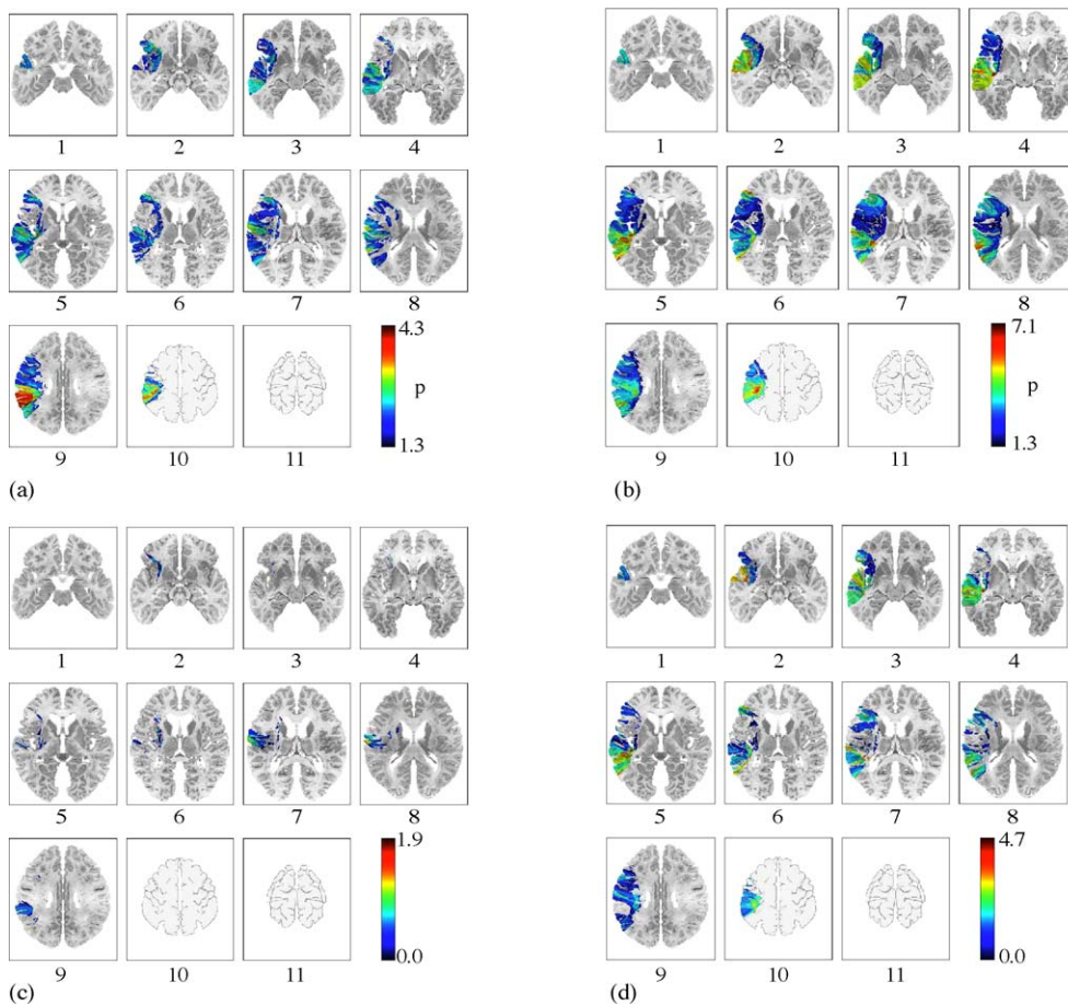
Fig. 3. VLSM maps showing significant foci associated with arithmetic performance (a) and comprehension (b). Voxels with larger p -values are plotted as hotter colors on the maps. p -values are in -\log_{10} scale. The bottom row shows VLSM subtraction maps for arithmetic minus comprehension (c), and comprehension minus arithmetic (d).
