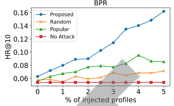
Fig. 4: Impact of the attack budget on the HR@10 for BPR.
