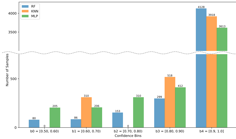
Figure 2: Classification confidence considering the features F1-F15.
